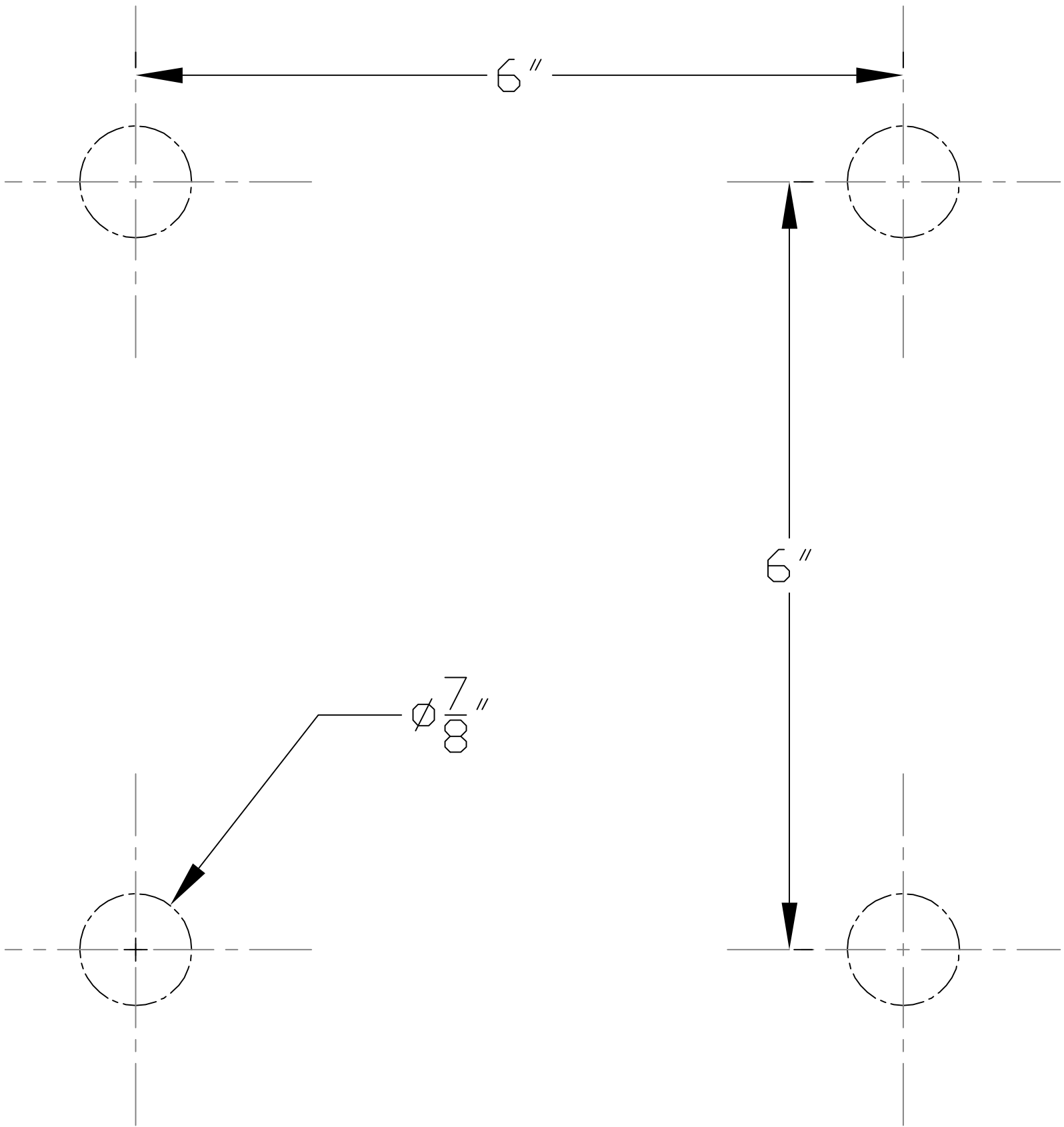
SIMME-SEAT EXPANSION ANCHOR TEMPLATE
