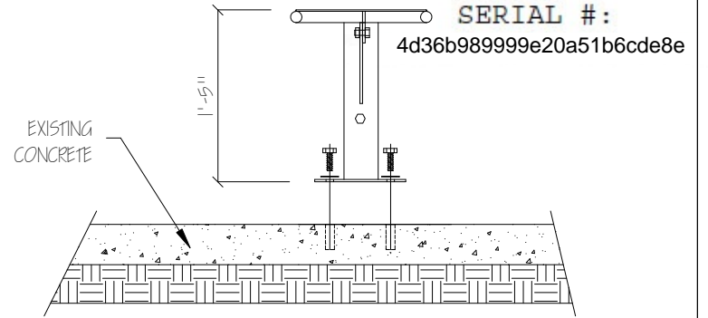
SIDE ELEVATION
