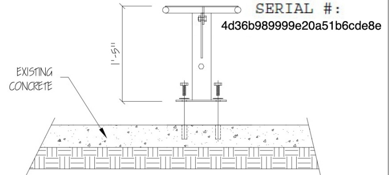
SIDE ELEVATION
