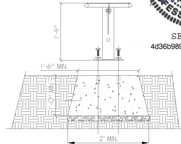
SIDE ELEVATION
